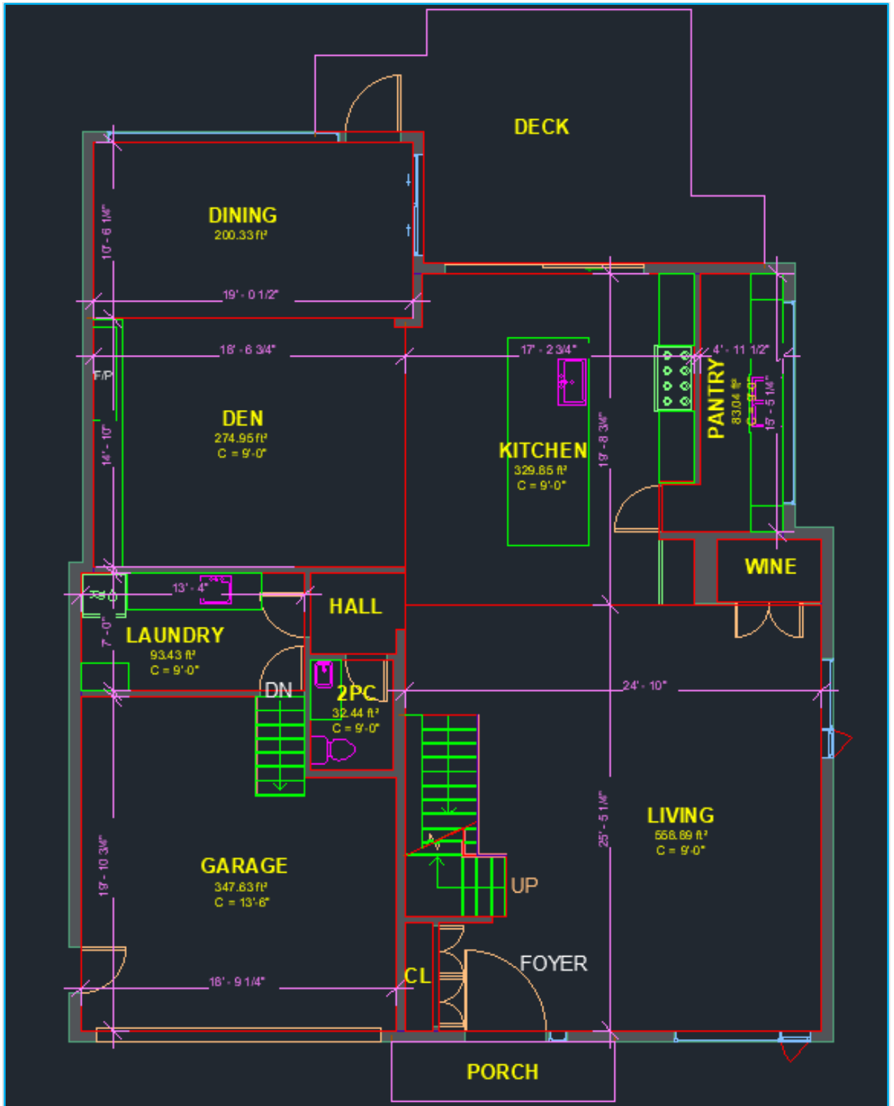
Image 8: Premium DWG Floor Plan
